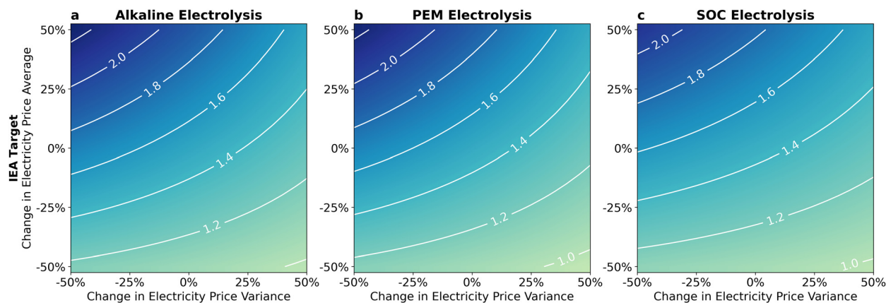
Fig. 5 Sensitivity of levelized cost of hydrogen estimates by 2030. This figure shows the sensitivity of our 2030 LCOH estimates to changes in the annual average and hourly variation of power prices for (a) alkaline, (b) PEM, and (c) SOC electrolyzers for the growth scenario postulated by the international energy agency (IEA).
